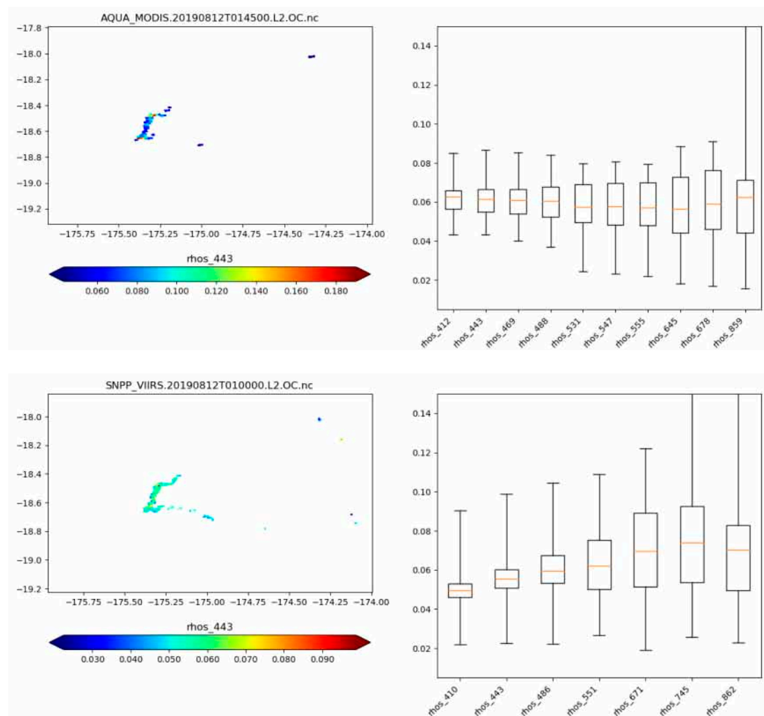
Figure 1. Left: Satellite \rho (rhos) reflectance data at 443 nm under the sea surface temperature (SST) mask of consolidated pumice for 12 August Coordinated Universal Time (UTC) from a threshold in Level 2 (L2) SST Moderate Resolution Imaging Spectroradiometer (MODIS) (top) and Visible Infrared Imaging Radiometer Suite (VIIRS) (bottom) data. Right: Satellite \rho (rhos) data of MODIS and VIIRS at different wavelengths under the “consolidated pumice raft”.
