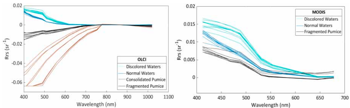
Figure 8. Spectra of Rrs pixels within surface pumice, discolored waters, and normal waters for (left) 9 August 2019 (21:33 UTC) using Sentinel-3A OLCI L2 Water Surface Reflectance at Full Resolution (WFR), and (right) 10 August 2019 (01:55 UTC) MODIS Aqua L2 data. Note that Rrs values were retrieved by dividing Oa3 reflectance (water-leaving radiance) values by \pi to make them comparable with MODIS values.
