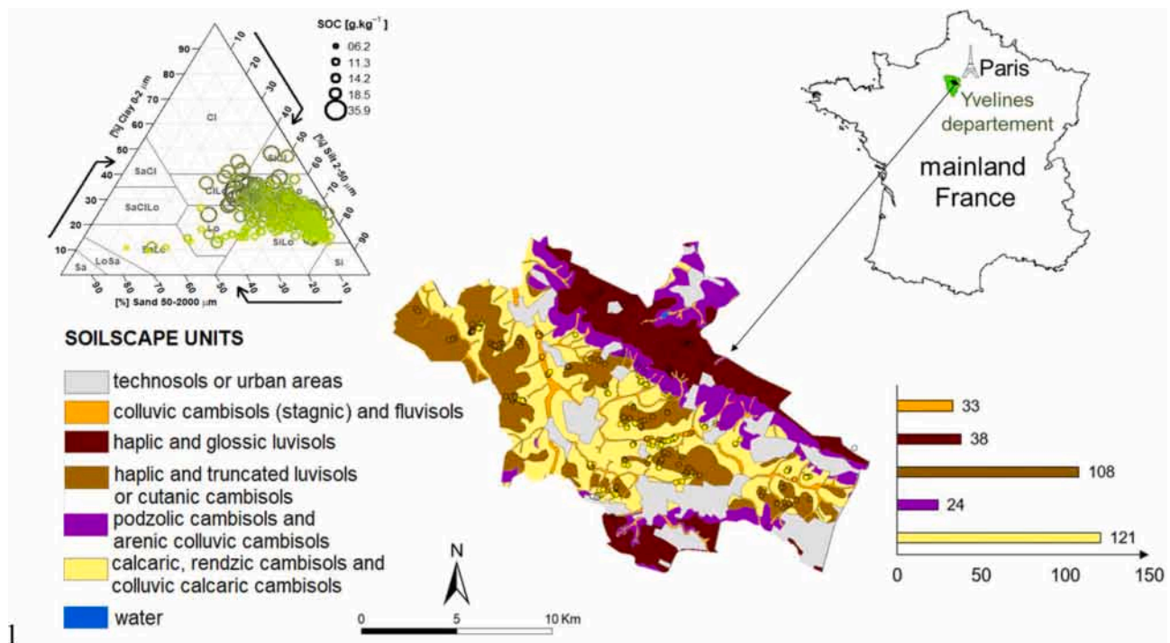
Fig. 2. Soilscapes map of the study area, main soil types and distribution of soil samples according to the soilscapes units and the soil texture triangle (larger circles indicate higher SOC contents).
