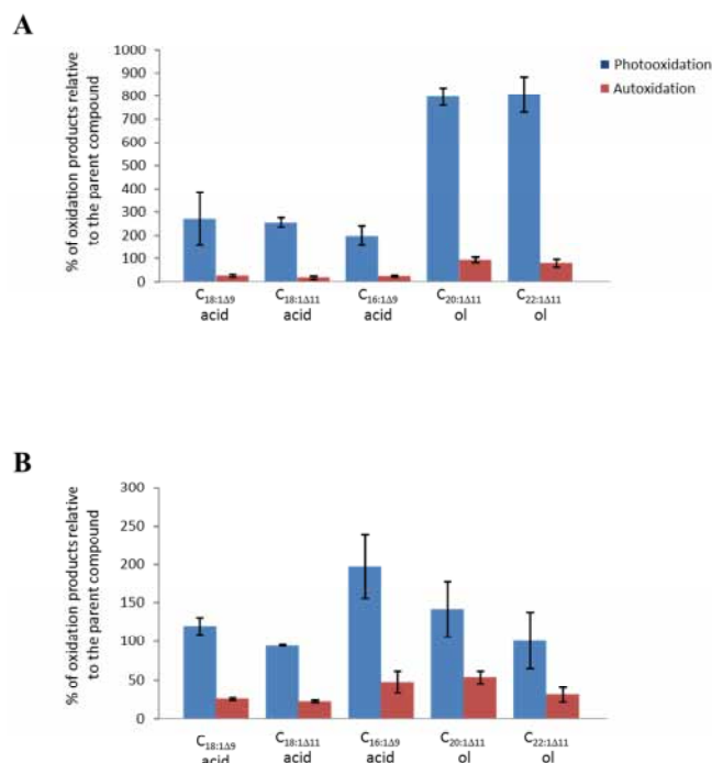
Fig. 3. Percentages of photooxidation and autoxidation products (relative to the residual parent compound) of monounsaturated fatty acids and alkan-1-ols observed in G09-A2 (A) and G09-A3 (B) samples.
