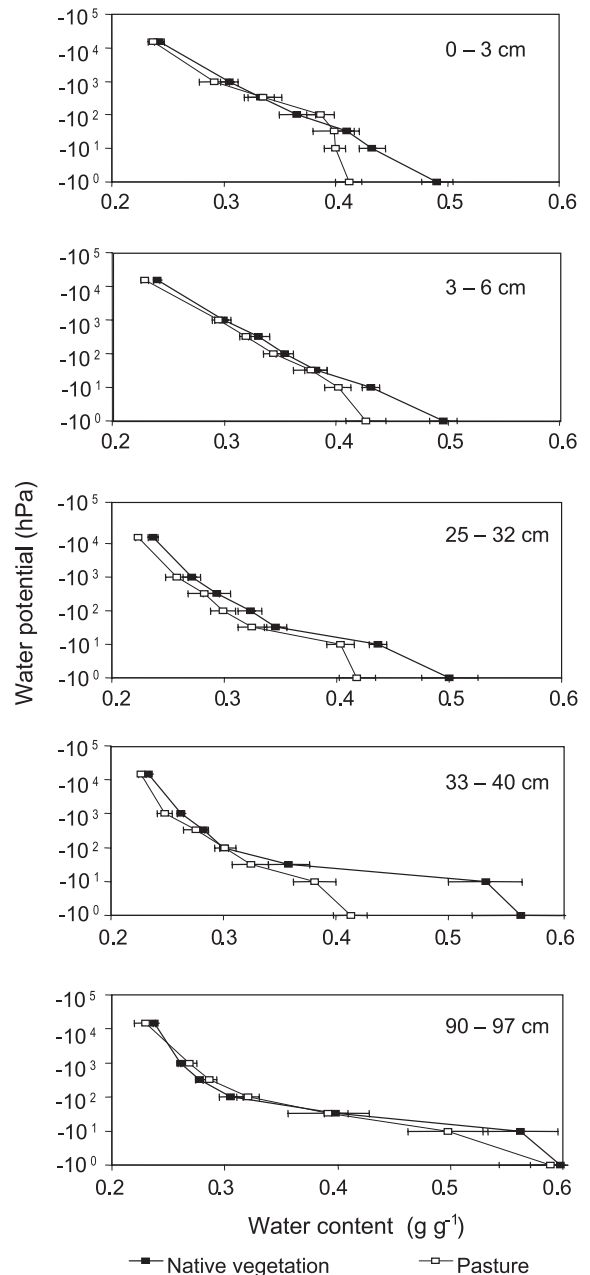
Fig. 2. Water retention properties measured using the small undisturbed samples collected under native vegetation and pasture (horizontal area \pm standard deviation).
