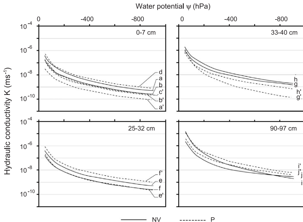
Fig. 3. Hydraulic conductivity, K(\Psi) , determined by using the evaporation method on core samples from the soil under native vegetation and under Pasture. (a, b, ..., i' and j' see Table 3 NV: Native vegetation; P: Pasture).
