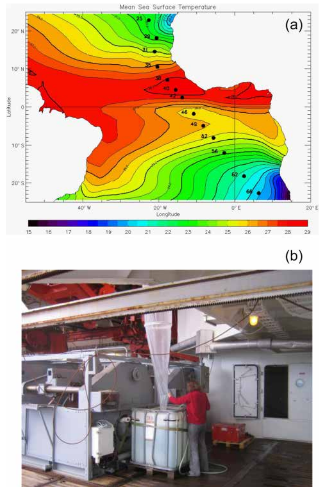
Figure 1. Stations used in this study plotted on gridded data set (Reynolds et al., 2002) (a). Setup for planktonic foraminifera collections (b).
