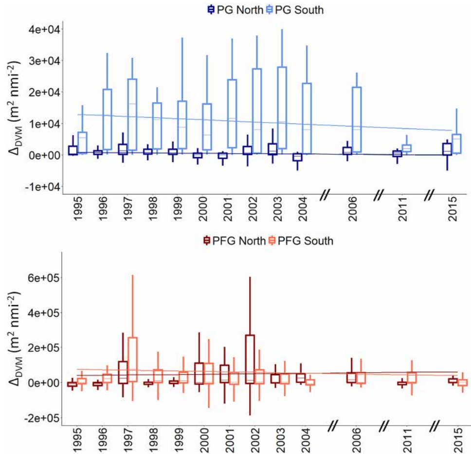
Figure 7. Differences to day and night acoustic density (Delta DVM, expressed in Nautical Area Scattering Coefficient notated NASC or s_A , m^2 nmi^{-2} ) for (top) the plankton group and pelagic fish group (bottom) echo classes in the areas north and south of Cap Blanc.
