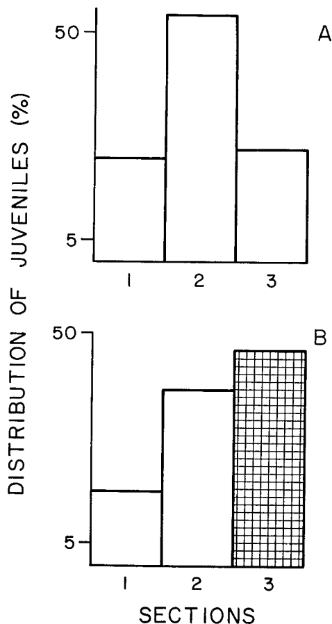
Fig. 2. Distribution of juveniles of M. incognita 48 h after their introduction in the center of section 2: A) in a column of sand mixed with 2.5% bentonite which was not used to grow tomato plants; B) in a column of sand mixed with 2.5% bentonite not used to grow tomato plants in sections 1 and 2 and with 2.5% bentonite used to grow 10 tomato plants for 7 d in section 3.
