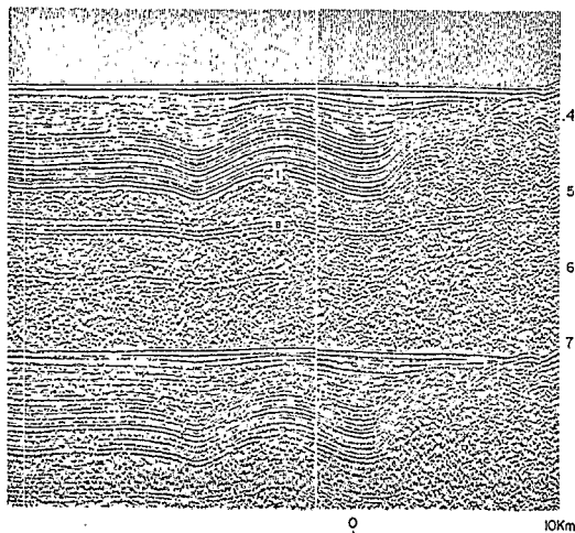
FIG. 2—Undulate structures from western Mediterranean Sea: T , roof of salt layer; B , floor of salt layer.
