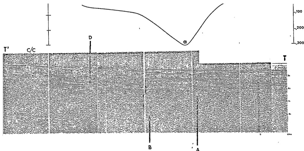
FIG. 7—T-T' section of Walda profile 18 (Fig. 5) showing southernmost diapiric structures. Rise of oceanic basement (A) marked by negative magnetic anomaly (a) of 300 \gamma is followed by its deepening under 3.5 sec of sediments (B). D is diapiric feature.
