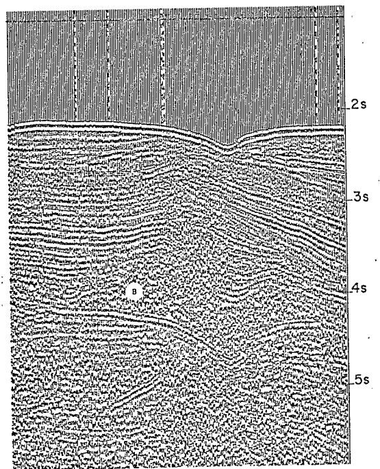
FIG. 3—Three types of salt structures: A, salt anticlines (X on Fig. 5); B, diapirs (U on Fig. 5); C, salt-injected fault (V on Fig. 5); with T, roof of salt layer, B, floor of salt layer.
