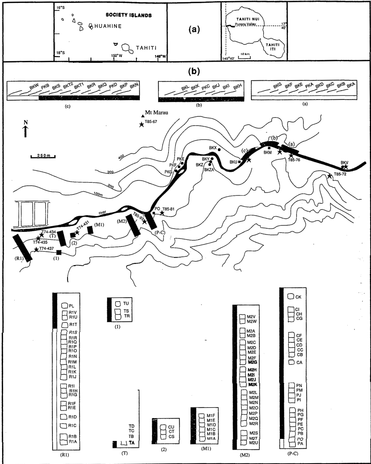
Fig. 1. a) Map of the Society islands (French Polynesia, south-central Pacific Ocean). The paleomagnetic sampling has been done along the Punaru Valley in the western part of the island of Tahiti (b). Flows are dipping toward the west. On the north side of the valley, the sampling was done along the river as indicated by the 3 sections a, b, c. Filled circles correspond to flows below (site BKV) and above sections a, b, c. Squares are the sampling sites of the dikes. On the southern border of the river, numerous cross sections of the hillside have been done and are indicated by letters referenced in the text. The magnetic polarity (black for normal) has been shown within each section. Gaps in the sampling are also indicated by discontinuities within each section. Stars correspond to the location of the dated samples.
