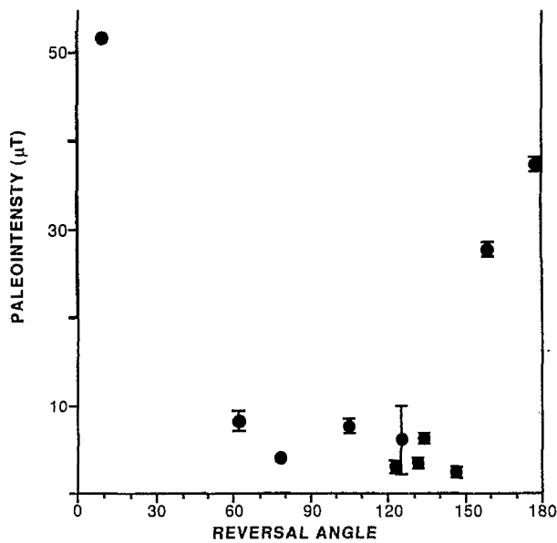
Fig. 14. Diagram showing the evolution of the mean paleointensities per flow with their standard deviations, versus the angular departure from the axial normal dipole. Paleointensities obtained from the intermediate flows are below 10 \mu\text{T} .
