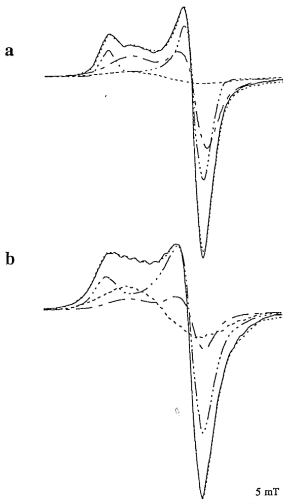
Figure 7. Least squares linear decomposition of the RID signal: — Experimental; ····· Fit; —·—·— A-center; --- A' center; - - - B-center (a) at 300 K for the kaolinite A1, (b) at 93 K for BAR kaolinite. The contents of the radiation induced defects are deduced from the proportion of the respective spectra.
