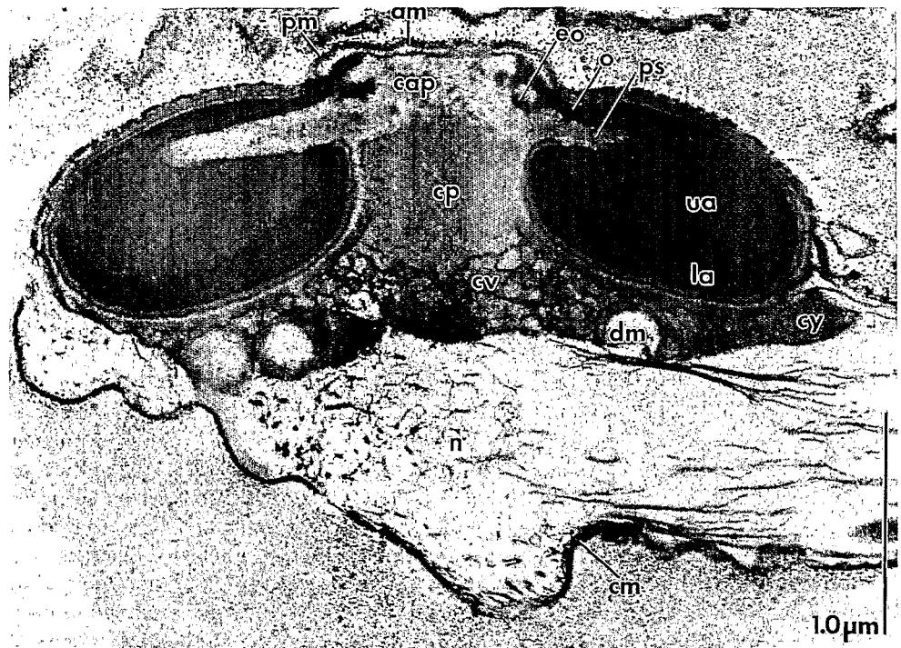
Fig. 2. Homologenus sp. Longitudinal section of a spermatozoon. am – acrosome membrane; cap – capitate region of perforatorium; cm – cell membrane; cp – core of perforatorium; cv – convoluted membranes; cy – cytoplasm; dm – degenerating mitochondrion; eo – extensions of the operculum into head of perforatorium; o – operculum; pm – plasma membrane; ps – perforatorial spike; ua – upper acrosomal zone
