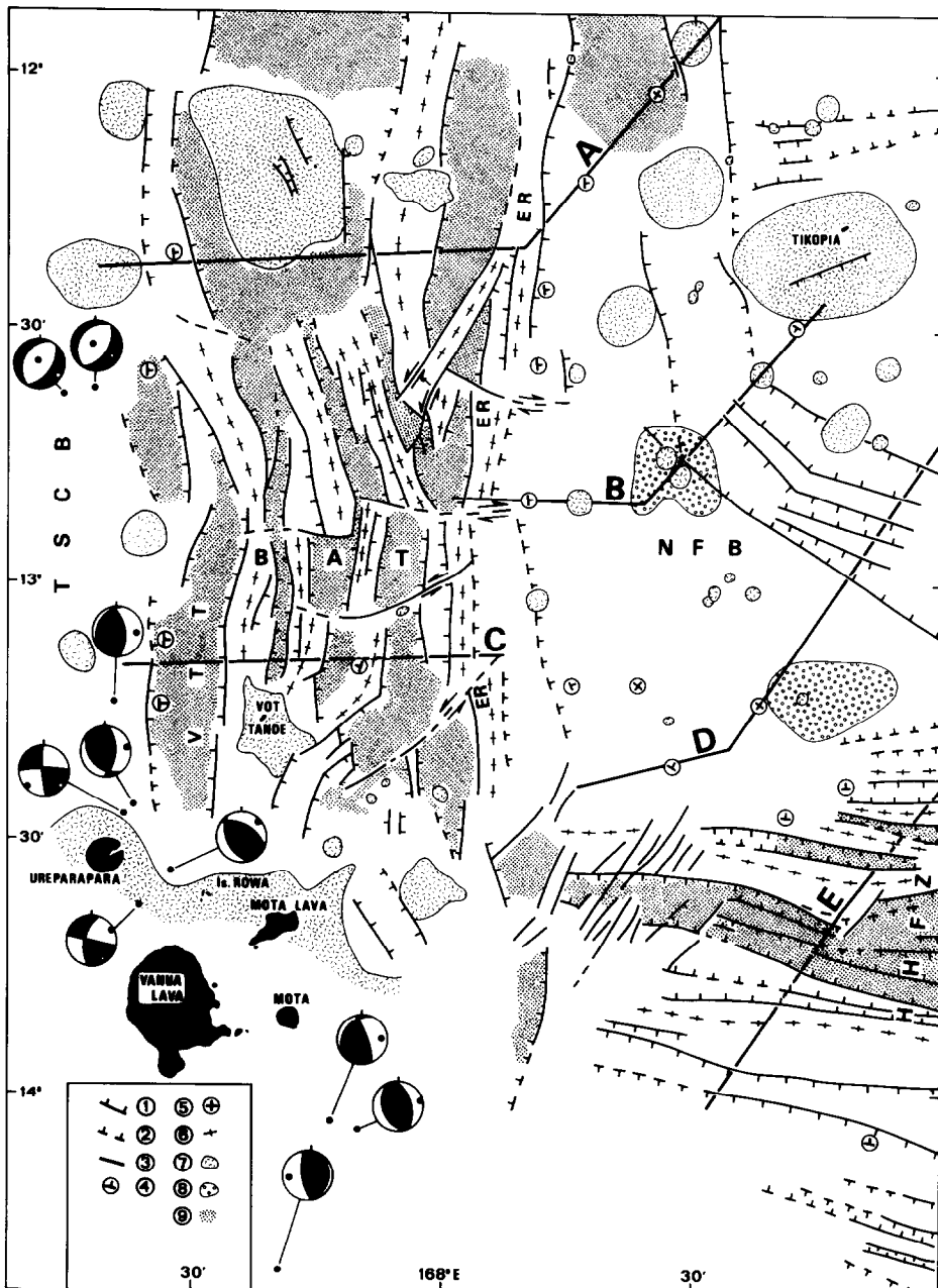
Fig. 4. Structural map of the northern New Hebrides back-arc troughs. 1 = normal fault; 2 = small and/or inferred normal fault; 3 = transverse tectonic lineation (arrows indicate strike-slip fault); 4 = inclined bedding; 5 = horizontal bedding; 6 = structural high; 7 = volcano; 8 = lava flows; 9 = major graben. TSCB—Torres Santa-Cruz sedimentary basin; BAT—back-arc troughs; VTT—Vot Tande trough; ER—Eastern Ridge; HHFZ—Hazel Home Fracture zone; NFB—North Fiji basin.
