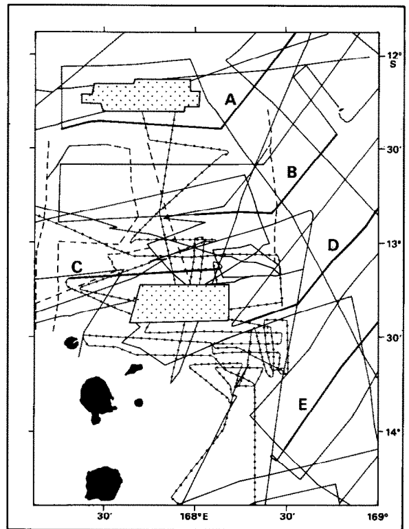
Fig. 2. Magnetic and bathymetric track lines used in this study. 1 = area of full Seabeam coverage; 2 = Seabeam and magnetic lines; 3 = bathymetric and magnetic lines; 4 = bathymetric lines; 5 = single channel seismic reflection lines shown in Figs. 5–9.
