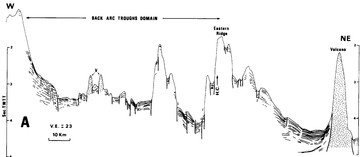
Fig. 6. Example of a seismic line bisecting the back-arc troughs in the northern part of the studied area (line A, location in Fig. 2). V—volcano; HC—heading change.
