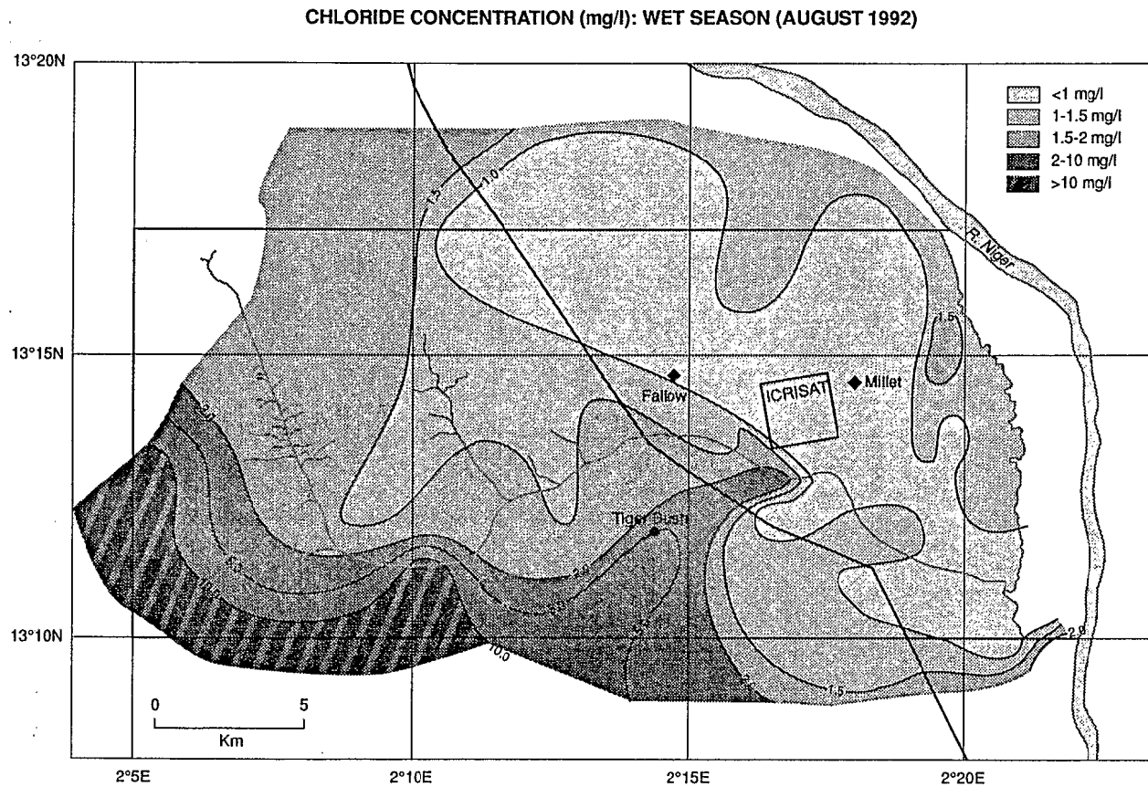
Figure 8. Distribution of Chloride during the wet season.
