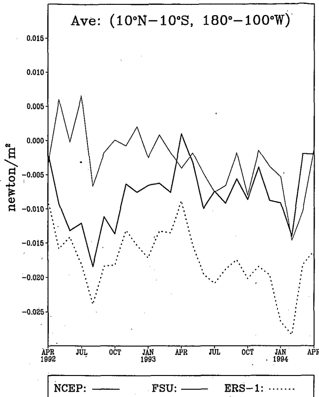
Figure 18. Zonal wind stress differences relative to TOGA-TAO for three products: NCEP, FSU, and ERS-1. The differences are averaged over 10°N to 10°S and 180° to 100°W. After Ji and Leetmaa [1997].
