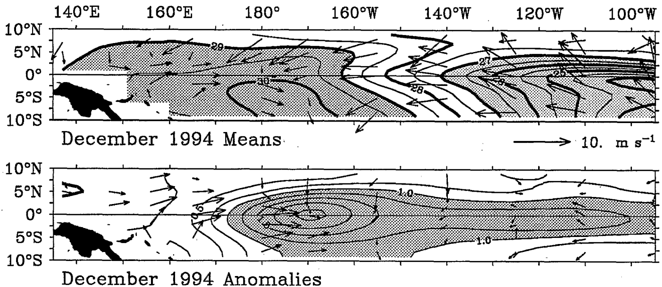
Figure 10. Wind vectors and SSTs from the TAO array for December 1994. (top) Monthly means; (bottom) monthly anomalies from the COADS wind climatology and NCEP SST climatology (1950–1979). SSTs warmer than 29^{\circ}\text{C} and colder than 27^{\circ}\text{C} are shaded; SST anomalies >1^{\circ}\text{C} and <-1^{\circ}\text{C} are shaded.
