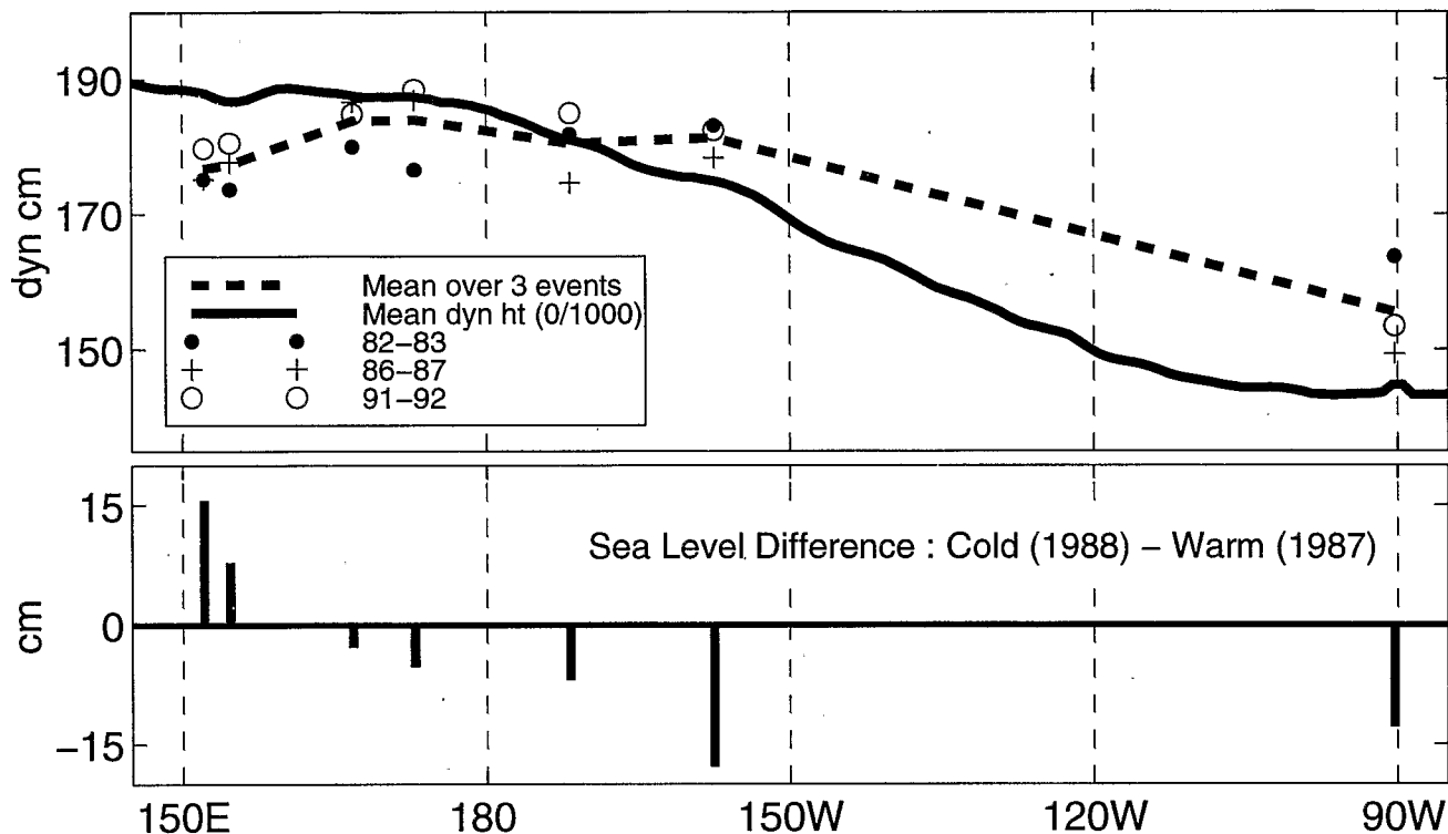
Figure 12. Zonal slope of sea surface height along the equator. Sea level anomalies from the 1975–1987 mean seasonal cycle were taken from seven locations near the equator: Rabaul ( 4^{\circ}\text{S} , 152^{\circ}\text{E} ), Kapingamarangi ( 1^{\circ}\text{N} , 155^{\circ}\text{E} ), Nauru ( 0.5^{\circ}\text{S} , 167^{\circ}\text{E} ), Tarawa ( 1^{\circ}\text{N} , 173^{\circ}\text{E} ), Kanton ( 3^{\circ}\text{S} , 172^{\circ}\text{W} ), Christmas Island ( 2^{\circ}\text{N} , 157^{\circ}\text{W} ), and the Galapagos Islands ( 0.5^{\circ}\text{S} , 90^{\circ}\text{W} ). These anomalies were added to the mean dynamic topography difference (0–1000 dbar) computed from the Levitus and Boyer [1994] and Levitus et al. [1994a] temperature and salinity climatologies in order to calculate absolute heights. (top) Mean conditions during three warm events are shown as solid circles (June 1982 to May 1983), crosses (January to December 1987), and open circles (June 1991 to May 1992). The heavy solid line is the long-term mean conditions taken from the Levitus climatology. (bottom) Warm and cold conditions are contrasted by showing the difference (the vertical bars) of the mean sea level anomaly in 1988 (cold) minus the mean sea level anomaly in 1987 (warm).
