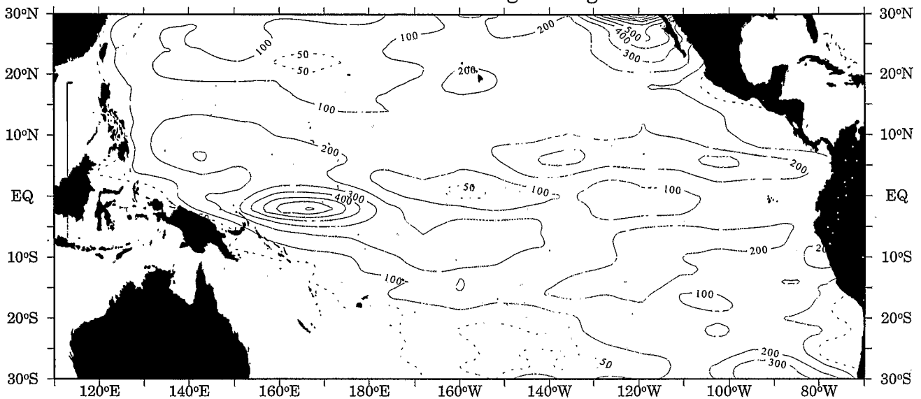
Figure B2. Number of 5-day observations of velocity observed in 2° latitude \times 8° longitude areas from surface drifters between January 1, 1979, and December 31, 1995, in the tropical Pacific. The total number of 5-day observations is 81,589. The maximum number of 5-day observations possible in any given box is 1098.
