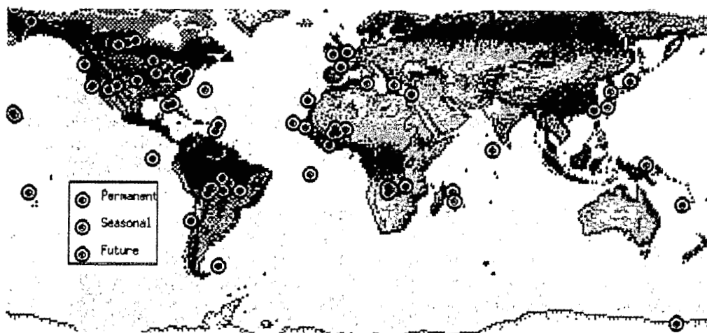
Figure 5. The approximate location of instruments is represented by the colored circles. Measurements are made at permanent sites year round. Data are taken seasonally at high latitudes and/or when cloud cover permits. In 1997 nearly 60 locations contributed to the database.
