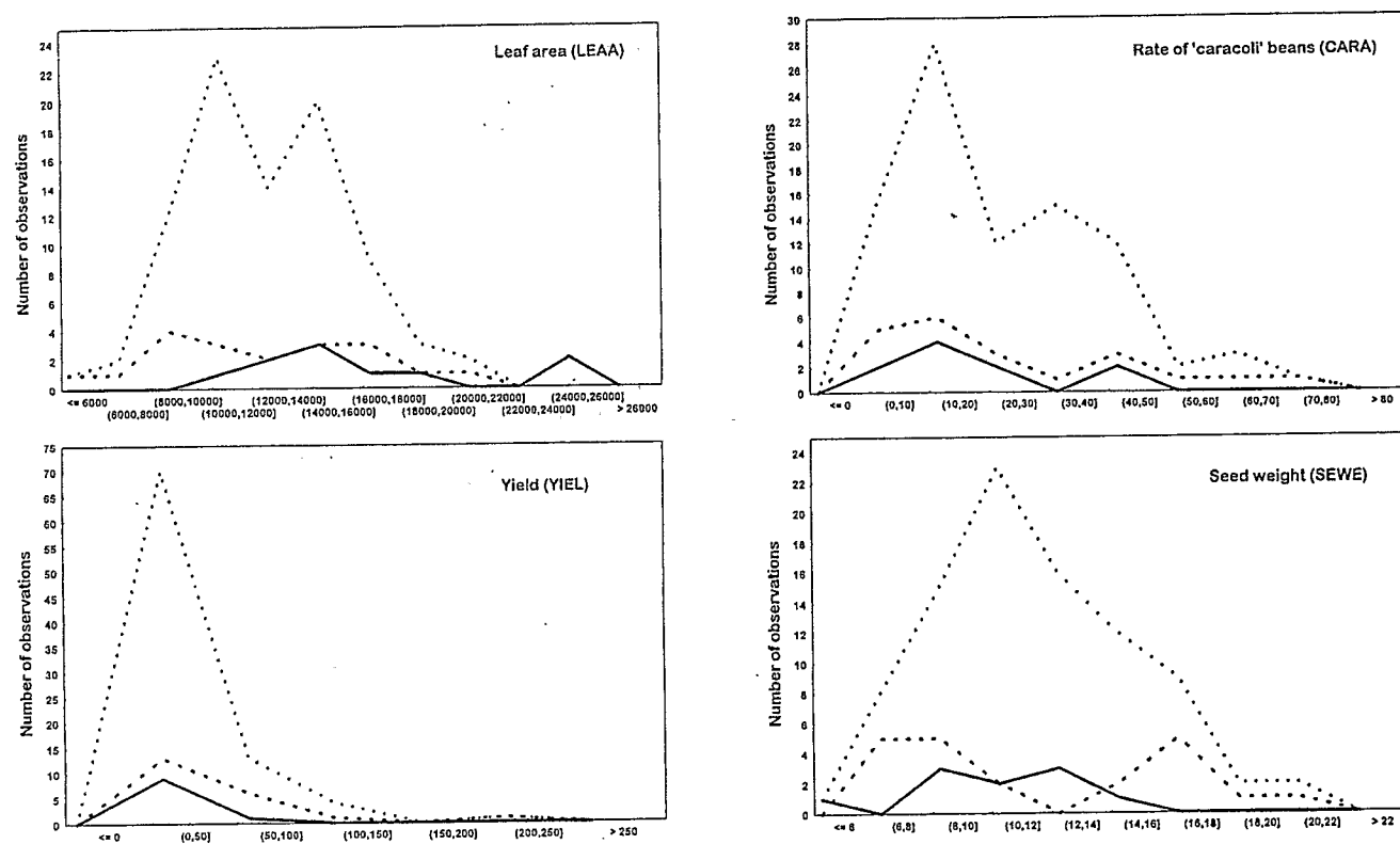
Figure 2. Coffee case. Distributions of leaf area, rate of caracoli beans, yield and seed weight in the base collection (dotted line), core collection selected on quantitative traits (hatched line) and in core collection selected with qualitative traits (solid line). Both core collections were defined by the 50 % cumulated contribution.
