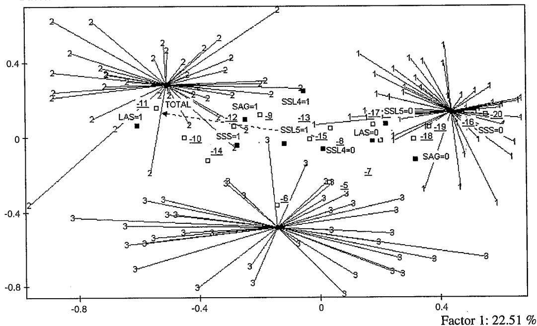
Fig. 7. First 2 axes of the correspondence analysis based on the structural descriptors of the diurnal scattering structures. Samples are grouped into 3 cluster analysis classes (1 to 3). Parameters (0: absence, 1: presence) on the figure are the only ones considered significant and useful
