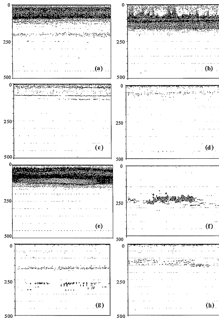
Fig. 2. Echotracés defined for the habitat characterisation. (a) 'Classic' sound scattering layer (SSL), (b) 'mountain' or inverse 'V' shaped scattering layer (MSL), (c) thin scattering layer (TSL), (d) loose scattering layer (LSL), (e) nucleus in scattering layer (NSL), (f) large aggregated structures (LAS), (g) stick shaped structures (SSS), (h) small aggregates (SAG)
