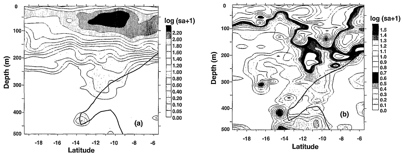
Fig. 4. Latitudinal vertical section of (a) nocturnal and (b) diurnal acoustic back-scattering by surface (sa) of micronekton on a logarithmic scale with the 1.5 \text{ ml l}^{-1} oxygen isoline plotted (solid line) on vertical section
