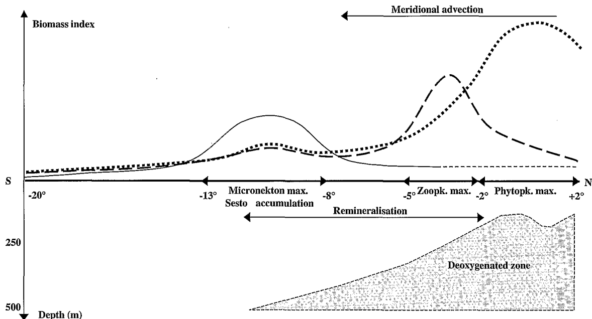
Fig. 12. Schematic representation of latitudinal distribution of phytoplankton (dotted line), zooplankton (dashed line) and micronekton (solid line) biomass in the 140°W zone with respect to latitudinal distribution of the deep deoxygenated zone during a positive Southern Oscillation Index (SOI) period
