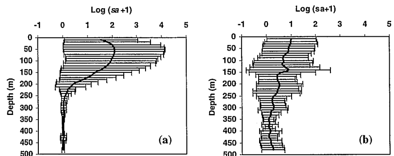
Fig. 3. (a) Nocturnal and (b) diurnal average profiles of acoustic back-scattering by surface ( sa ) of micronekton with their profiles deviation on a logarithmic scale
