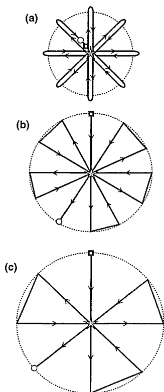
Figure 2. Survey patterns used during acoustic surveys around FADs in French Polynesia. ★, FAD position; □, start of the survey; ○, end of the survey.
