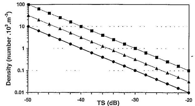
Figure 7. Minimal densities (number · 10^3 \cdot m^{-3} ) for echo integration as a function of mean target strength (TS) values for three integration thresholds ( S_v ): -60 dB (—■—), -65 dB (—▲—) and -70 dB (—●—).
