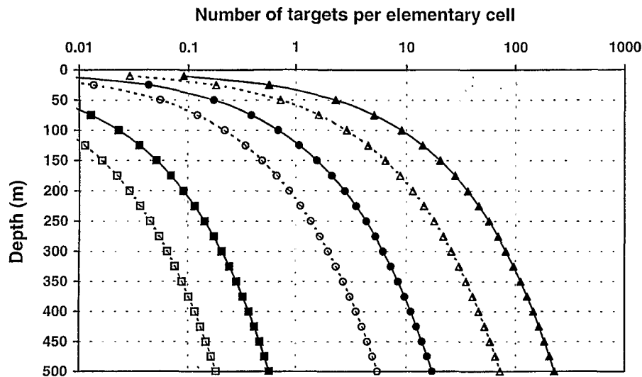
Figure 8. Minimum number of targets per elementary units for echo integration for different integration thresholds ( S_v ) and target strength (TS) values. —▲—, S_v = -60 dB, TS = -46 dB; —●—, S_v = -60 dB, TS = -34.8 dB; —■—, S_v = -60 dB, TS = -20 dB; —△—, S_v = -65 dB, TS = -46 dB; —○—, S_v = -65 dB, TS = -34.8 dB; —□—, S_v = -65 dB, TS = -20 dB.
