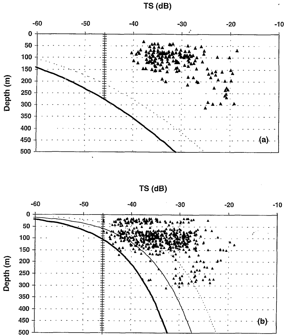
Figure 5. Acoustic limits of the echo sounder in (a) echo-counting (individual target detection mode); and (b) echo integration at a vessel speed of 7 knots. a) Echo-counting: ·····, theoretical maximum depth to detect an individual target located outside the acoustic axis, at the maximum angle authorised for the detection of an individual target; ———, theoretical maximum depth to detect an individual target located in the acoustic axis; +++++, threshold value used to extract target strength (TS) data with the EP500 software; ▲, (TS–depth) data from echo-counting. (b) Echo integration: ·····, Sv threshold = -60 dB; ———, Sv threshold = -65 dB; ———, Sv threshold = -70 dB; +++++, threshold value used to extract target strength (TS) data with the EP500 software; ▲, (TS–depth) data observed during echo integration.
