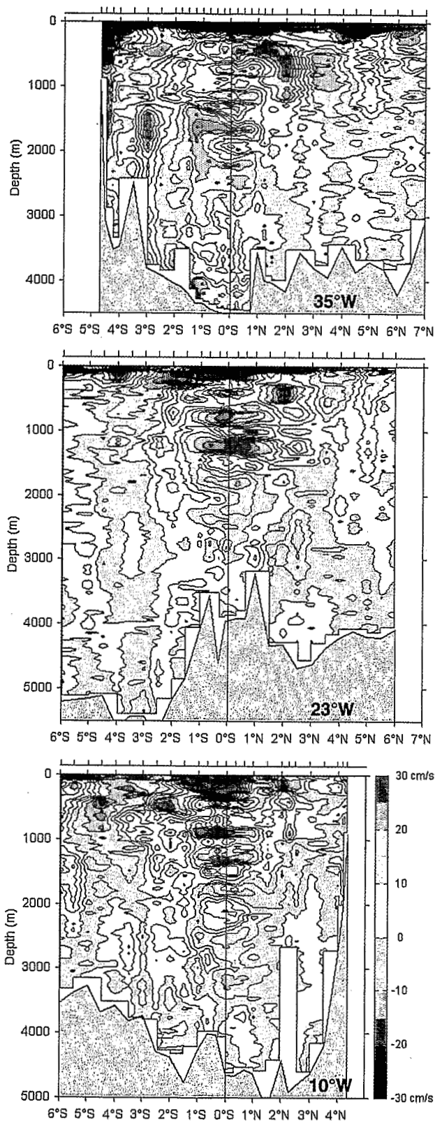
Plate 1. Latitude-depth section of the zonal component of velocity, in \text{cm s}^{-1} , along 35^\circ\text{W} , 23^\circ\text{W} , and 10^\circ\text{W} . Eastward (westward) currents are positive (negative). Contour interval is 5 \text{ cm s}^{-1} . Station positions are reported on the top of every section.
