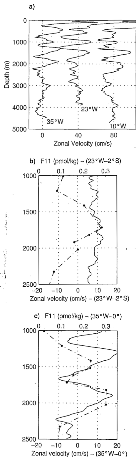
Figure 2. Vertical profiles of CFC-11 and LADCP measurements. (a) Depth profiles of the zonal component of velocity in \text{cm s}^{-1} , at 35^\circ\text{W} - 0^\circ , 23^\circ\text{W} - 0^\circ , 10^\circ\text{W} - 0^\circ . Each profile has been shifted by 40 \text{ cm s}^{-1} from the preceding one. Eastward (westward) currents are positive (negative). (b) CFC-11 profile (dashed-dotted line) and zonal velocity profile (solid line) at 23^\circ\text{W} - 2^\circ\text{S} . (c) CFC-11 profile (dashed-dotted line) and zonal velocity profile (solid line) at 35^\circ\text{W} - 0^\circ . The detection limit for the CFC-11 measurements was about 0.009 \text{ pmol kg}^{-1} .
